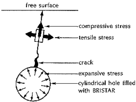
Fig.4:Fracture Mechanism by the expansive stress of BRISTAR
