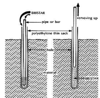
Fig. 8: Use of Polyethylene Sack in hole
